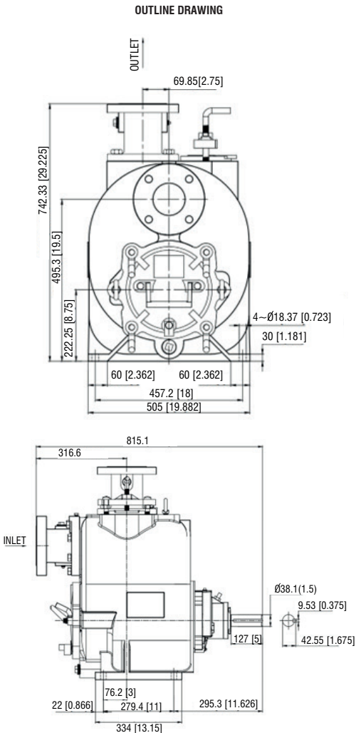
Figure 1. Pump Model ESPT4
