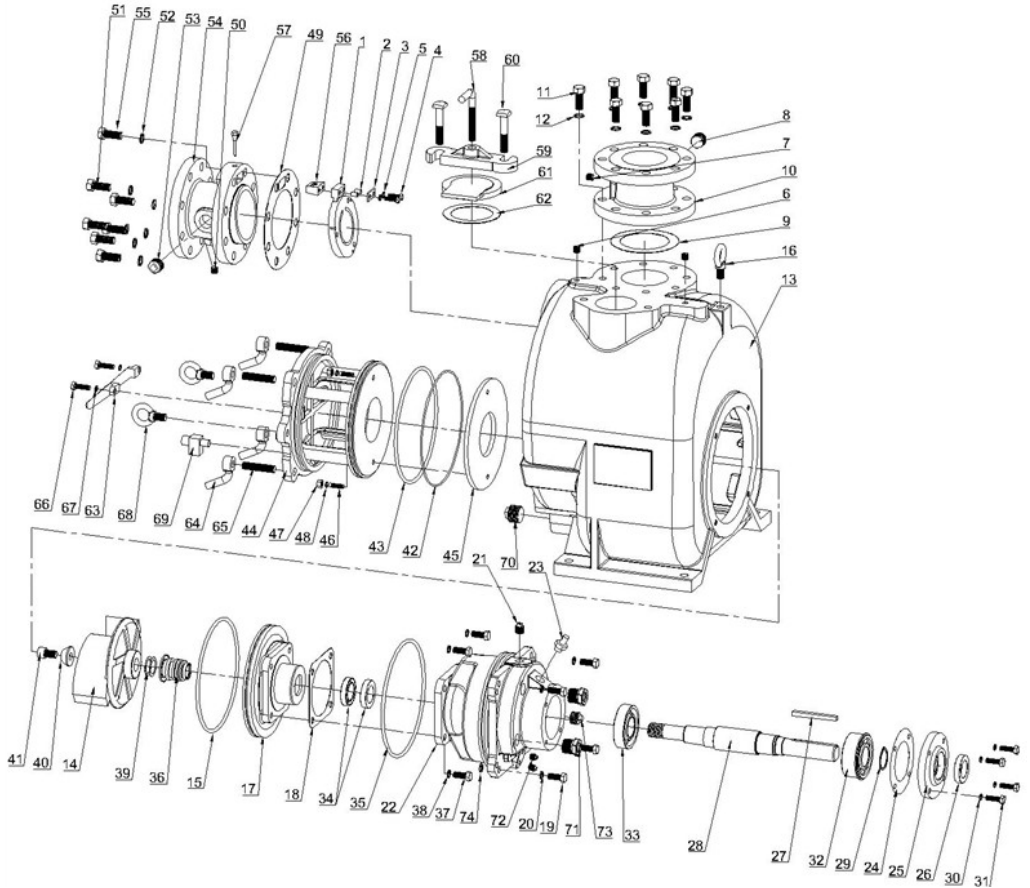
* Figure 1. Pump Model ESPT4
