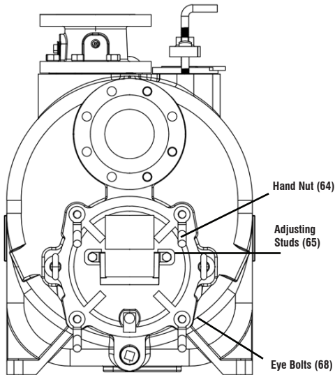
Figure 7. Installing and Adjusting Back Cover
