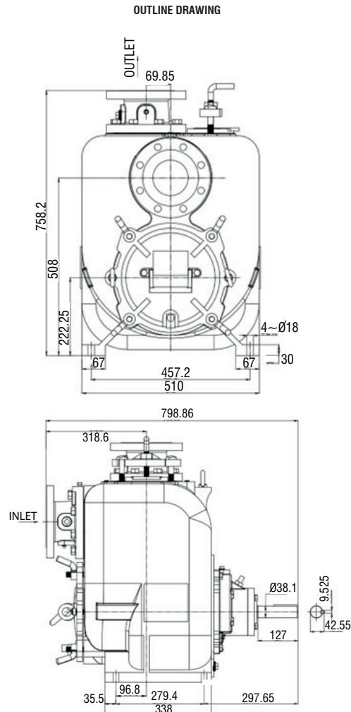
Figure 1. Pump Model ESPU3
