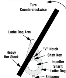
Figure 2. Loosening Impeller
