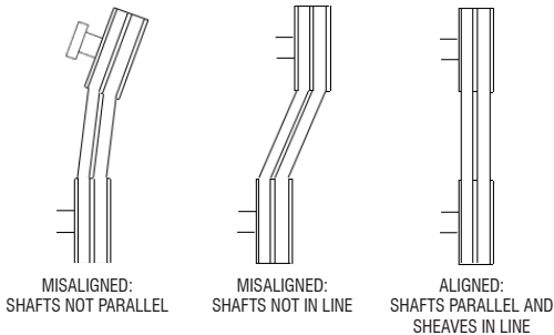
Figure 7. Alignment of V-Belt Driven Pumps
