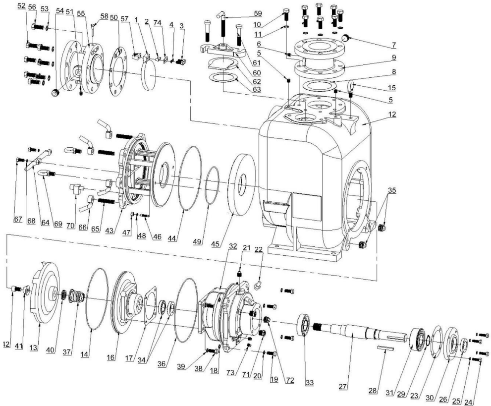
* Figure 1. Pump Model ESPU4
