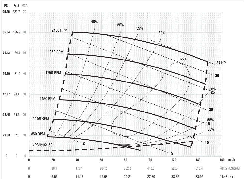
PERFORMANCE CURVE MODEL ESPU4
