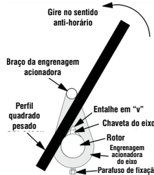
Figure 2. Loosening Impeller
