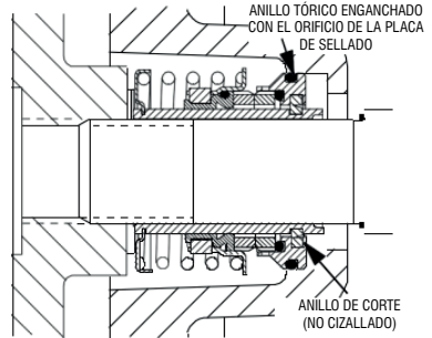
Figure 5. Seal Partially Installed
