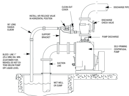
Figure 4. Typical Automatic Air Release Valve Installation
