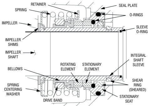
Figure 4. Cartridge Seal Assembly
