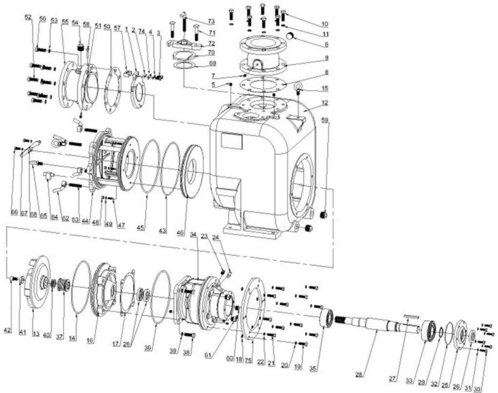
* Figure 1. Pump Model ESPU6
