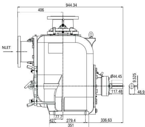
Figure 1. Pump Model ESPU6
