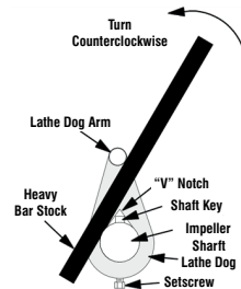
Figure 2. Loosening Impeller
