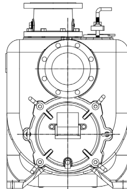
Figure 7. Installing and Adjusting Back Cover
