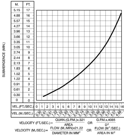
Figure 2. Recommended Minimum Suction Line Submergence vs. Velocity
