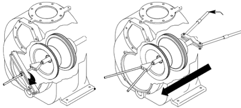
Figure 3. Rotating Assembly Removal
