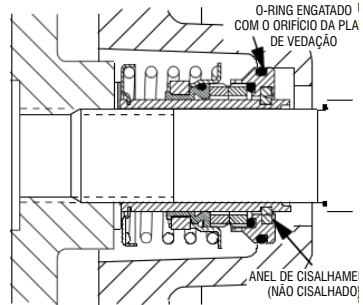
Figure 5. Seal Partially Installed
